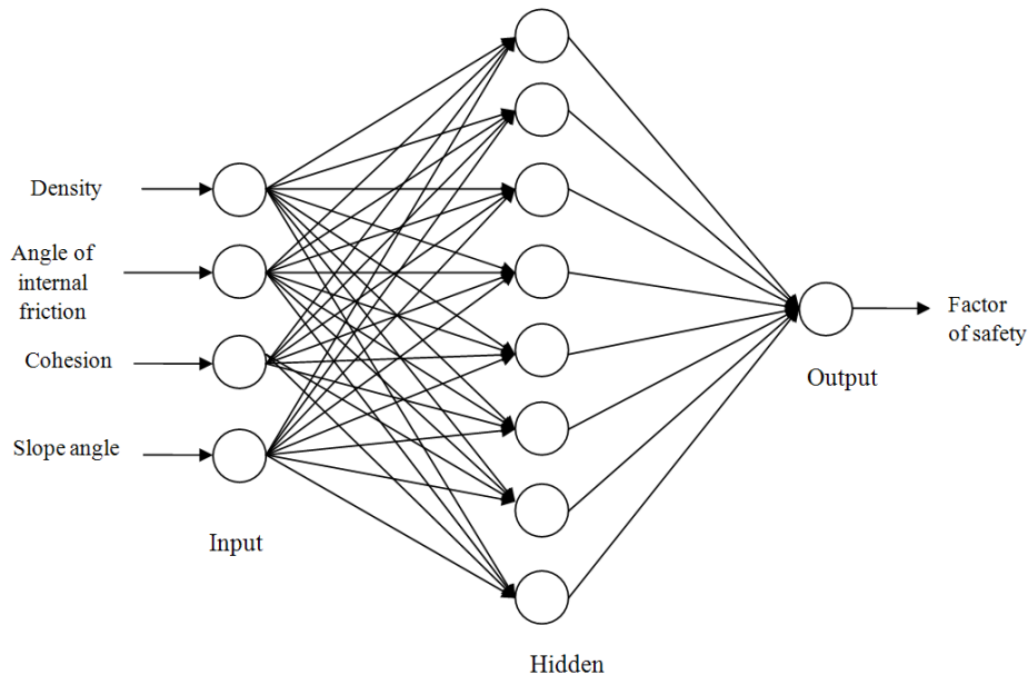
Fig. 3. BP-ANN architecture
