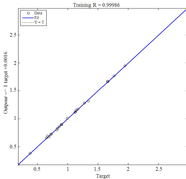
Fig. 5. Regression plot between target values Vs predicted values
