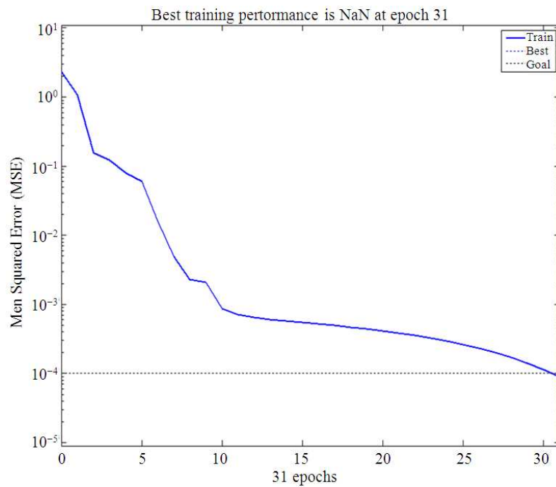
Fig. 4. BP-ANN Training performance graph (MSE Vs Epochs)
